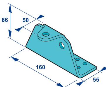
12 trous Ø 12 mm
